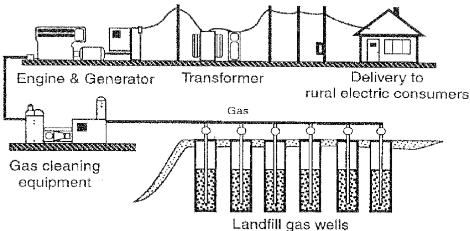
Simplified Plan of Coffin Butte Resource Project
