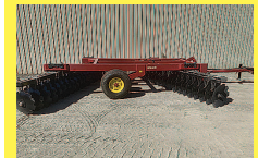
NEW IA Heavy Duty Offset Wheel Discs. Scraper kit, EZ adjust gang angle, split gang axles, 26" notched blades front and rear. •9ft. $12,400 •10ft. $12,900 •11ft. $13,400 •12ft. $13,900 •13ft. $14,400 •14ft. $17,900 •15ft. $18,900 •16ft. $19,900 •18ft. $21,900 8ft.-22ft. 8,000 lbs. Introductory pricing. Order NOW! Bend, OR. 541-548-7185 mtcsales.net
