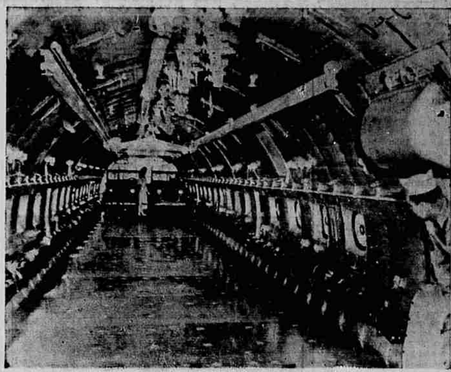
GLOBEMASTER'S INTERIOR HAS SPACE FOR 30 TONS—World's largest land plane, the giant Douglas C-47 Globemaster, has interior large enough to accommodate two army jeeps side by side. Ship has overall length of 124 feet, cargo load of 30 tons, maximum range of 7,800 miles, enabling it to fly around world with but two stops. New features are built-in freight elevator, traveling cranes, reversible propellers enabling ship to taxi backwards into hangers.
