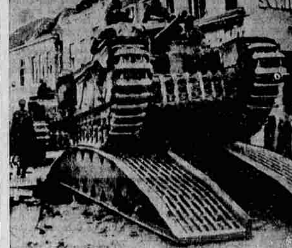
BRIDGE ON TANK—TANK ON BRIDGE—The photos above are the first released of the British army's "Scissors" tank, which carries its own bridge with it. From a normal position on the top of the tank, the bridge portion is lifted by a hydraulic arm, as shown in top photo, and deposited across narrow streams. The bottom picture, made in Holland where narrow streams and canals abound, shows the bridge in use.
