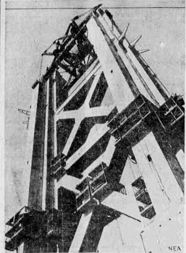
Here's a new angle on bridge construction—the way the mighty tower of the Golden Gate bridge looks to a fish or a boatman in San Francisco Bay. The tower is rising on the Marin county side, to support what will be the world's largest suspension bridge.
