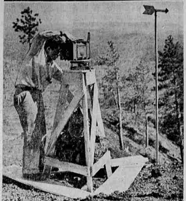
A special type of camera devised for photo survey work, is being used by the forest service in visual mapping, with oriented exposures being made from every lookout station in Oregon and Washington.
