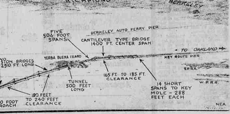
This preliminary sketch of the final design for the $75,000,000 San Francisco bay bridge has been prepared for study and approval of the state director of public works for California.
