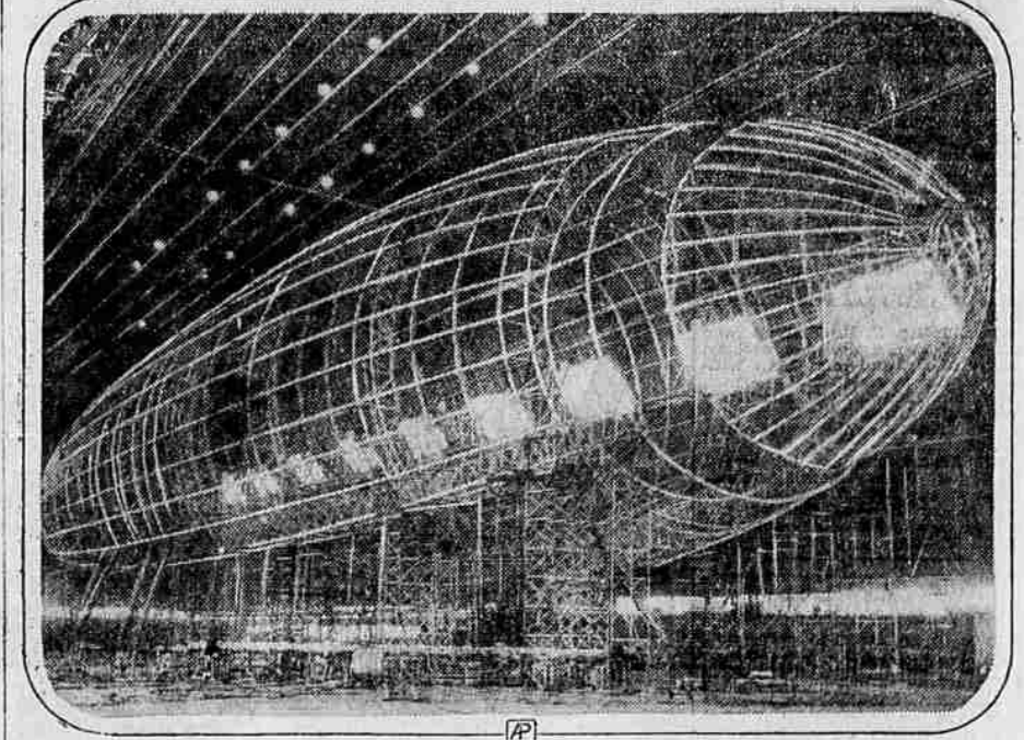
The metal skeleton of the first of the two new super-dirigibles being built for the United States navy is now being covered with fabric, in preparation for test flights in June. The new dirigible has a gas volume nearly twice that of the Graf Zeppelin.
