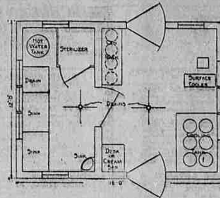
MODERN MILK HOUSE Floor Plan
