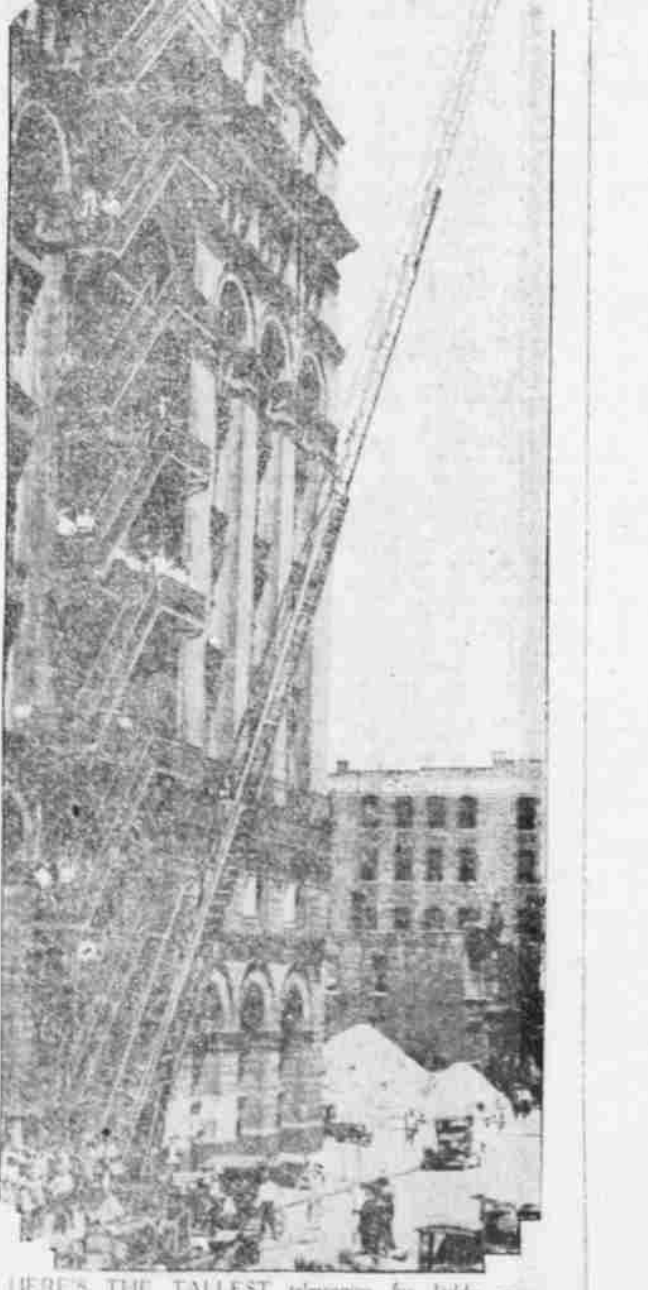
HERE'S THE TALLEST telescoping fire ladder in America, undergoing tests by the Milwaukee fire department. The ladder is raised to its maximum height of 100 feet, which can be done in 30 seconds. It was made in Germany.
