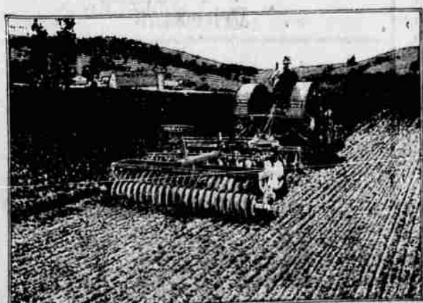
McCormick-Deering 4-cylinder FARMALL, the new all-purpose tractor for planting and cultivating row crops. Leads the way to real horseless farming.
