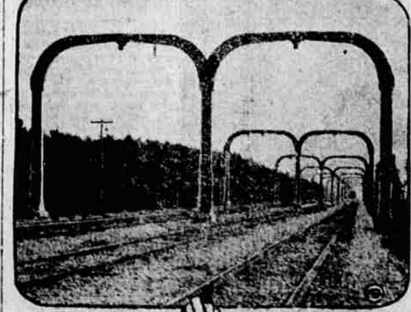
Railway men throughout the country are watching with interest Henry Ford's experiment of electrifying his railroad. The Detroit, Toledo and Ironton Photo shows a stretch between Dearborn and Flat Rock, Mich., where electrification is complete. The big arches carrying the power wires are made of concrete, come in two pieces, and Ford has built a special factory to make them. He will install them eventually all along the line.
