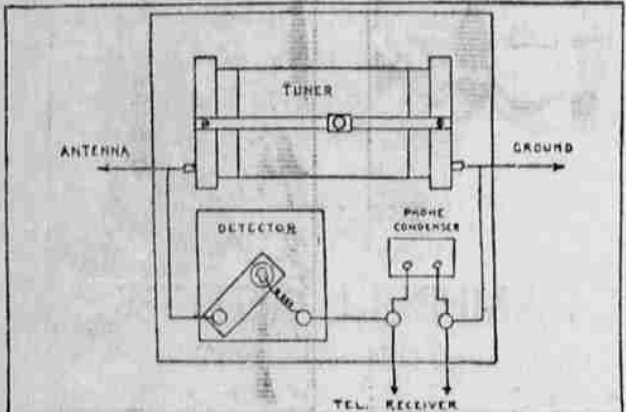
Set Mounted on Base, With Connections Shown.
