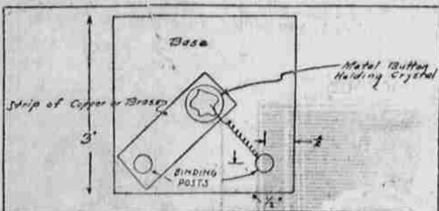
The Crystal Detector.
