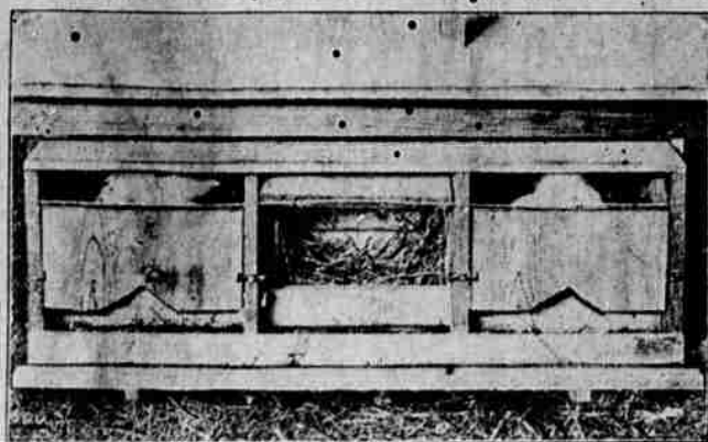
Three-Compartment Trap Nest Is Not Difficult to Make.
