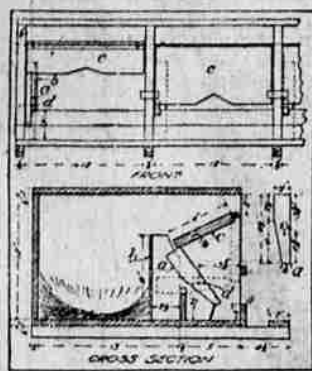
Details of Construction of Trap Nest.
