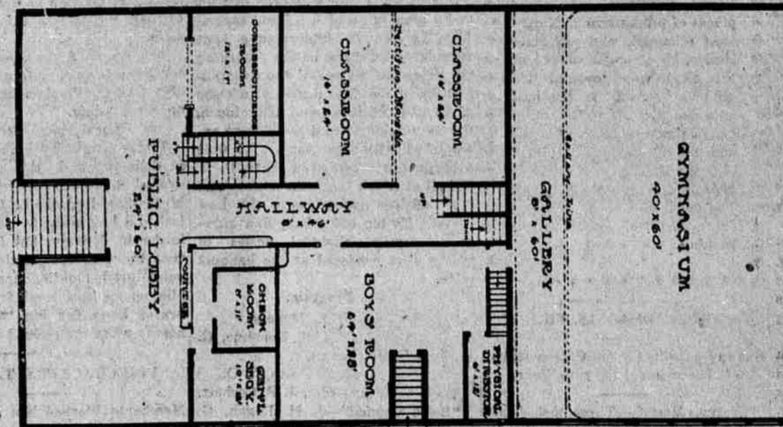
Main floor of building likely to be located at Elm and Washington.
