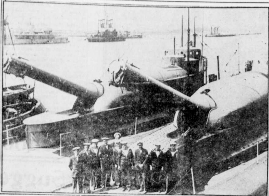
The latest British submarines armed with 12-inch guns which can be submerged fully loaded, capable of firing torpedoes, under water, and able to dive completely under the surface of the water in 15 seconds.
