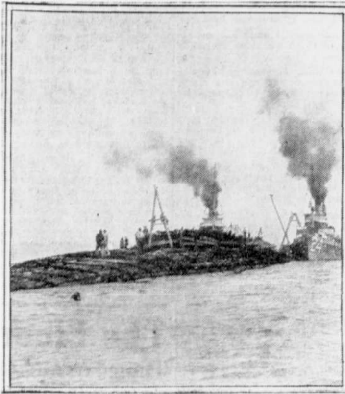
Aided by two U. S. Navy Mine Sweepers the largest log raft ever built, ended its voyage successfully by sea from the Columbia river to San Diego, Calif., recently. The log raft approximately 200 feet long, broke loose twice and was on the verge of going ashore and breaking up. Besides "carrying itself" it served as a barge, carrying a million shingles, a half million lath and 30,000 feet of telegraph poles.
