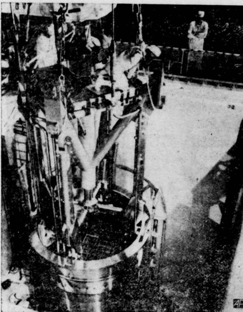
AN ATOMIC FUEL CHARGER is lowered into the giant 58-ton cone containing an atomic fuel charge at the Duquesne Light company plant at Shippingport, Pa. The plant is to begin generation of electricity late this year.
