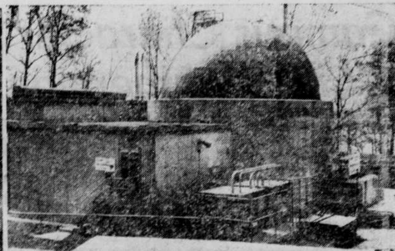
ATOMIC PLANT TO BE DEDICATED —The Army (April 23) permitted news photographers to visit this atomic power plant which will be dedicated at Ft. Belvoir, Va., next Monday. It is called a "package" plant because it is designed so that its components may be transported by air for installation at remote military stations, such as Arctic bases. The output, 1855 kilowatts, will be distributed as available on the Ft. Belvoir electrical system.
