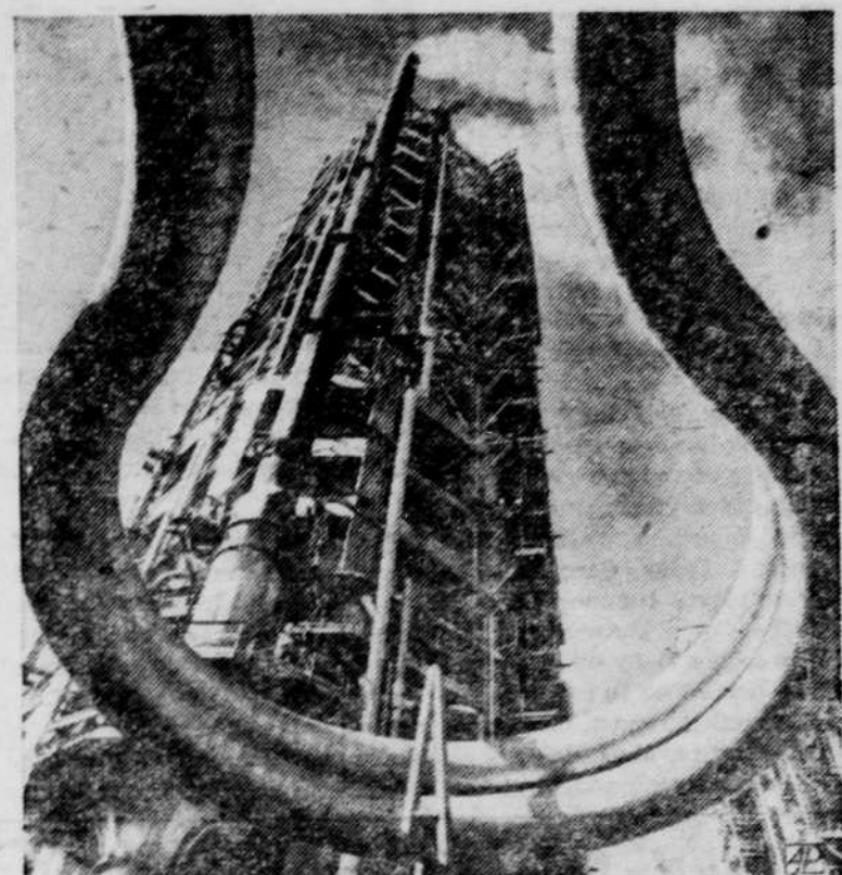
NEW TEXAS GIANT —Steam line expansion loop frames latest Texas skyscraper, a 330-foot wall, 28,000-barrels-per-day catalytic cracking unit, put into operation at Beaumont.
