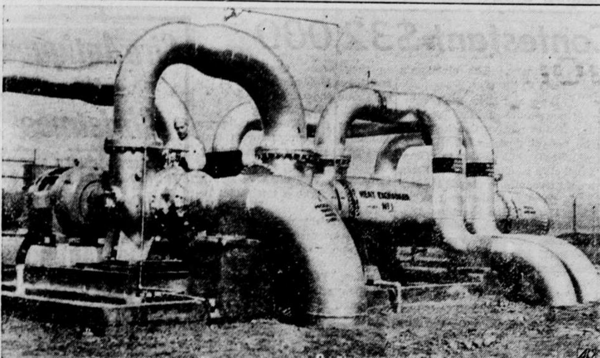
THIS IS PART of the atomic heating system now keeping buildings warm at the Hanford atomic plant at Richland, Wash. The maze of pipes transfer heat from water used to cool atomic reactors to the air conditioners in various nearby buildings. It is the first such heating unit of its kind in this country. (AP Wirephoto.)
