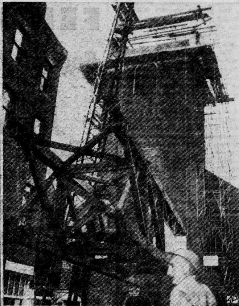
A CRANE LIFTS SUPERSTRUCTURE of new Old North Church steeple from truck as it starts to raise it to the tower of the church in Boston, Mass. The steeple will replace the one toppled by hurricane Carol last year. Reconstruction is expected to be completed in August. (AP Wirephoto)
