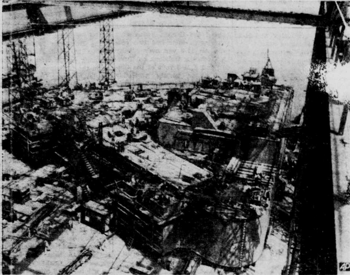
THE FIRST OF THE OFFSHORE radar plane-detecting towers is nearing completion at the Fore River shipyard at Quincy, Mass., and will be launched soon. The huge, triangular shaped steel platform, weighing 2000 tons will be towed to sea and placed in position on caissons in the ocean on Georges Banks, about 110 miles east of Cape Cod, Mass. The towers will make up a radar chain stretching along the Atlantic coast from Norfolk, Va., to Newfoundland, a distance of 1500 miles. (AP Wirephoto)
