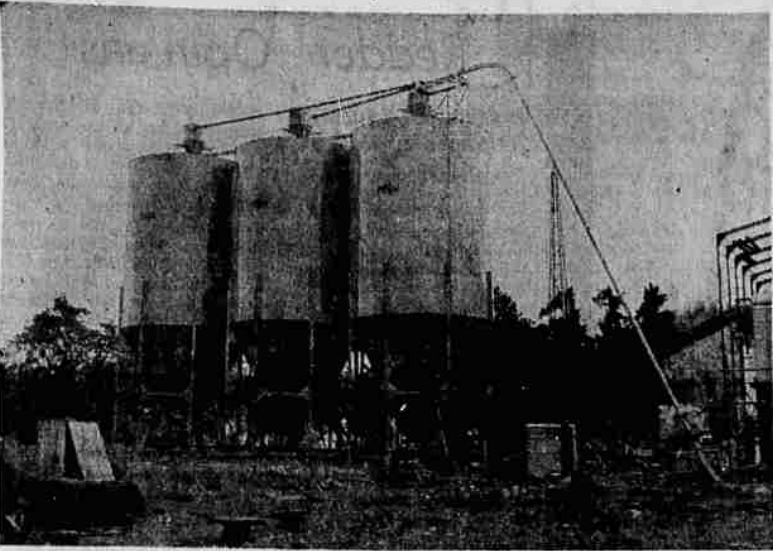
FUEL STORAGE SILOS — Three steel fuel silos, pictured above, have been built at the Martin Bros. Container and Timber Products Corp. plant in Oakland by Sutherlin Machine Works, Inc. The silos are 32 feet in diameter, 72 feet high and have total capacity of 570 units of hogged fuel.
