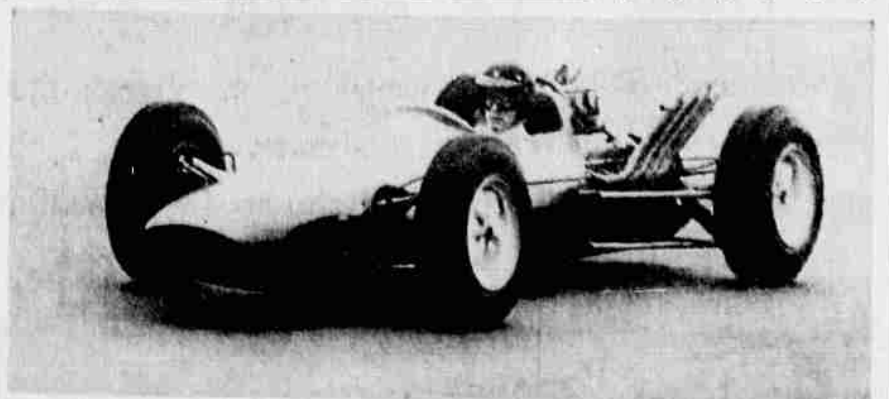
THE BOMB — Racing driver Don Gurney test drives prototype of a new model from Lotus Cars Ltd. of England at the Indianapolis Speedway. The car was built specifically for the Indianapolis 500. It has a 350-hp horsepower Ford aluminum V-8 engine in the rear. (UPI Telephoto)
