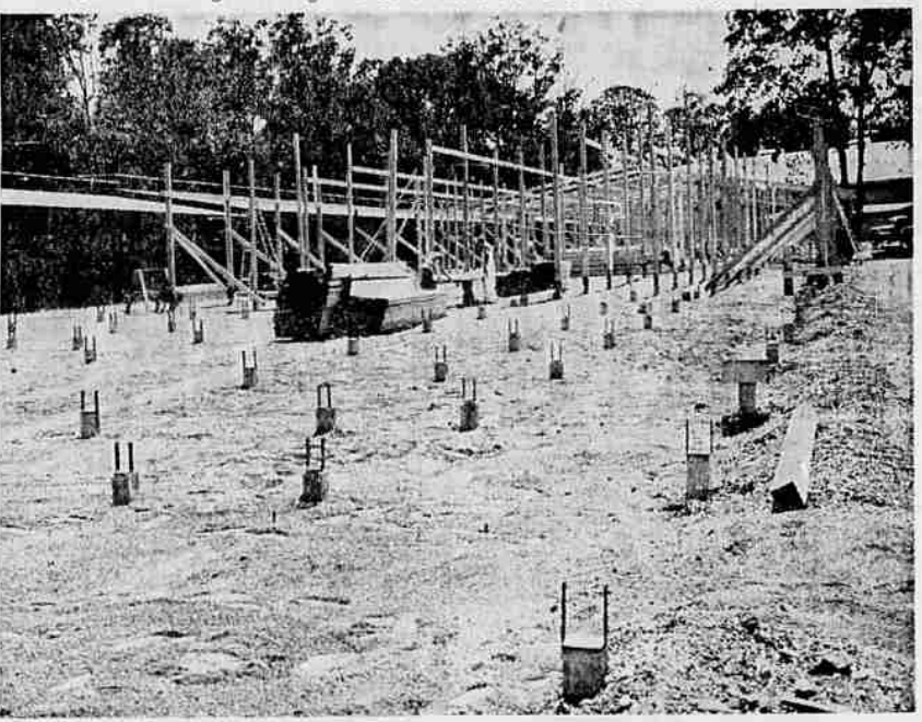
MAJOR CONSTRUCTION project at the Fairgrounds this year is this new livestock barn. Paralleling the existing barn, it is 372 feet by 58 feet. Its construction allows an expansion of the open class in livestock. James & Stritzke of Roseburg is doing the construction. (News-Review Photo).
