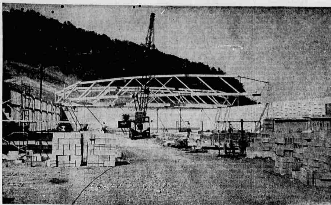
GIANT TRUSSES , 96 feet in length, went up Thursday morning to form the roof supports for the new Indian Lanes bowling alley, now under construction to the north of Roseburg's city limits. Jay Oldham's crane equipment was called here from Eugene to put up the glue-laminated beam trusses, which eliminate need for supporting posts. They were produced by Truss Fab, Inc., Portland. Short-
