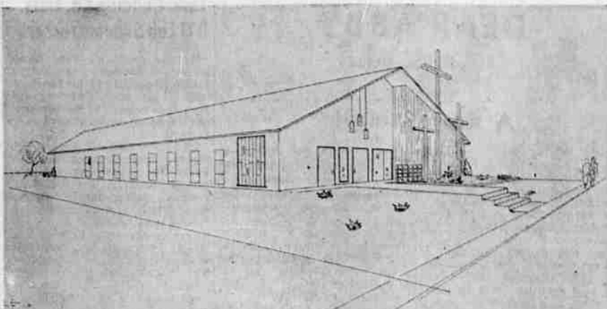
PICTURED ABOVE is an artist's sketch of the new sanctuary for the Church of the Open Bible, for which ground breaking services are scheduled Sunday. This will be a part of the Easter Sunday festivities at the Church. Construction is scheduled to get under way early next month. The design is by Mel Hanson, Portland.
