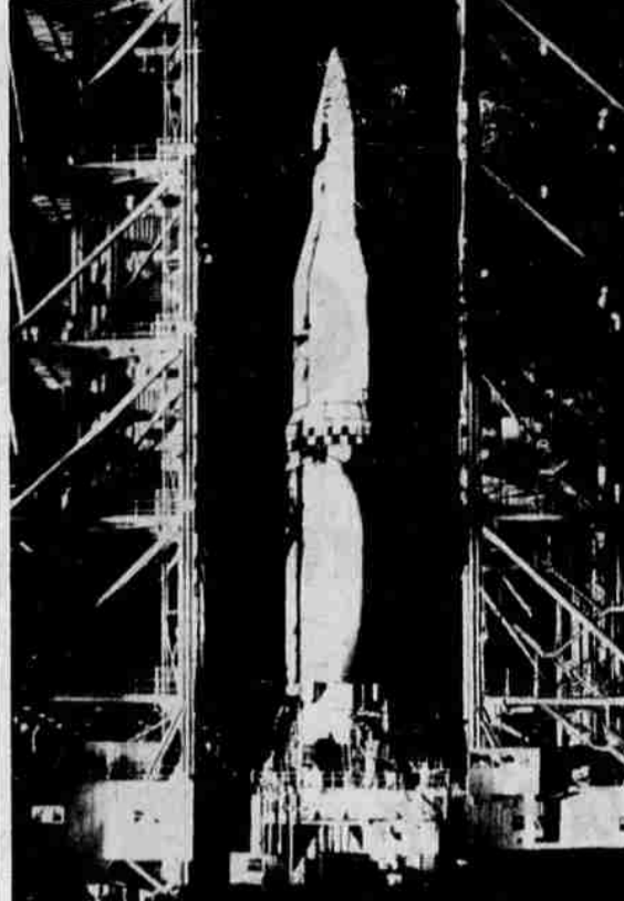
LAUNCHING NEAR — Saturn, the largest U. S. space vehicle ever developed, will be launched in the very near future, it was announced Wednesday by the National Aeronautics and Space Administration. The vehicle is shown at Cape Canaveral, Fla., being readied in the gantry that is 185 feet high, the world's tallest structure on wheels. The Saturn will have 1.5 million pounds of thrust. (UPI Telephoto)
