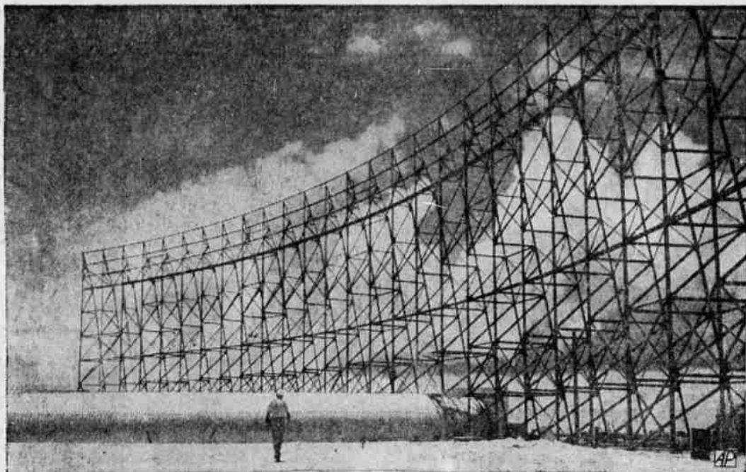
PACIFIC DEFENSE LINK—This is the shielding fence to deplete lethal radio frequency waves generated by transmitter at the Zeus Acquisition Radar (ZAR) center on Kwajalein atoll. Metal tunnel extends from fence to transmitter building.
