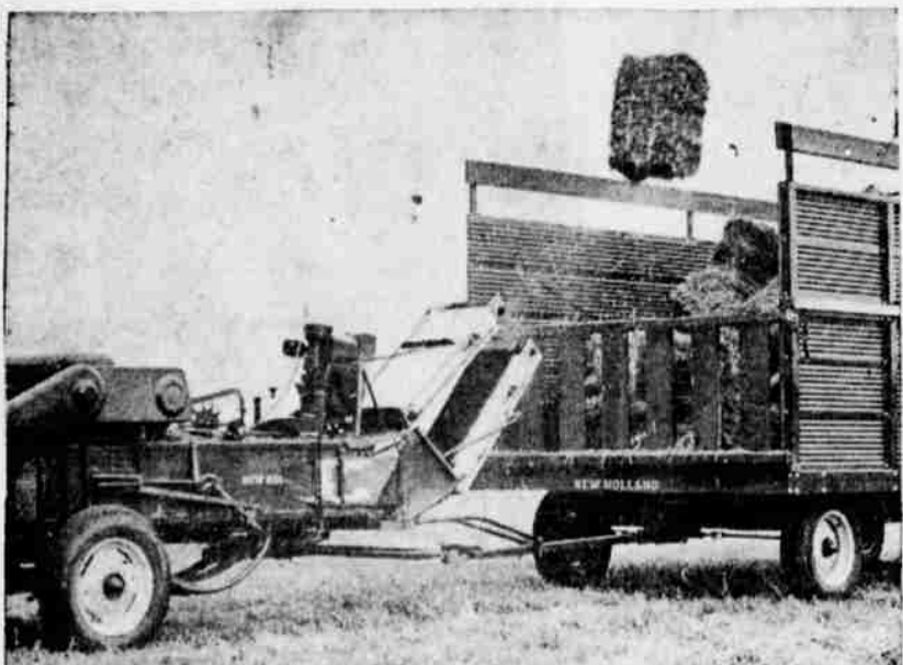
PERFECT PITCH—An experimental device that tosses hay bales from the baler to the farm wagon with big-league-pitcher accuracy is shown being demonstrated at New Holland, Pa. It removes the toil from one of hay-making's toughest jobs. The bale thrower is operated from the tractor by a throttle controlling the thrower's engine. Between the white "jaws" seen at end of baler are two high-speed belts which constitute the "pitching arm."
