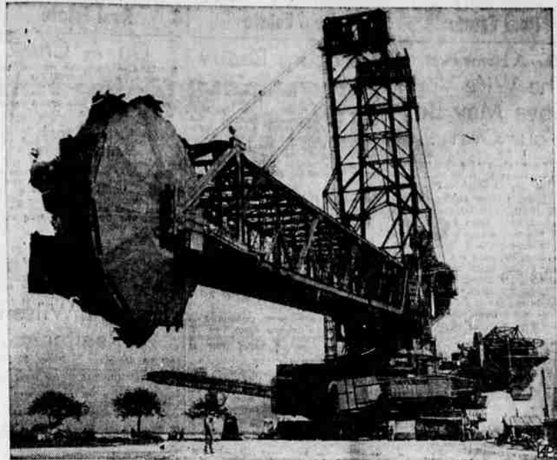
GIANT ON THE MOVE —This 6,000-ton dredging machine looms above the landscape at Duerrwis, Germany, as it lumbers under its own power to a nearby job. The huge digger, built in two years, has an overall length of more than 500 feet and is over 200 feet high.
