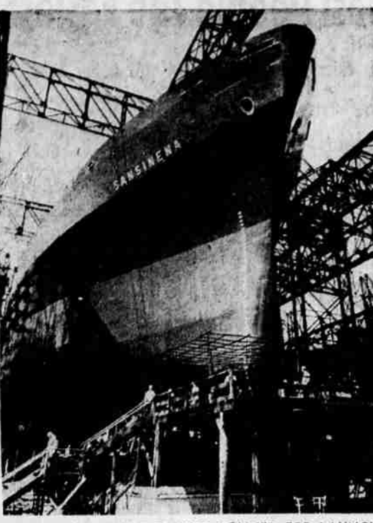
BIGGEST U. S. BUILT TANKER READIED FOR LAUNCHING — The 810-foot Samsinena, capable of carrying 20,580,000 gallons of oil, gets final touches in Newport News, Va., shipyard for launching Aug. 7. It is the largest tanker ever built in the United States. It towers 10 stories above its keel and is more than three city blocks long. The Union Oil Company of California will operate it under charter between the west coast and Persian Gulf. (AP Wirephoto)
