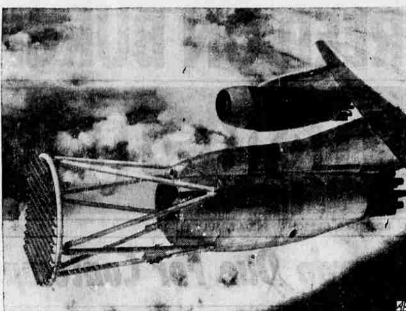
TEST IN THE CLOUDS — Lattice device sprays water into engine of Boeing airliner in high altitude de-icing test. Jet engine's hot air melted ice in less than 30 seconds.
