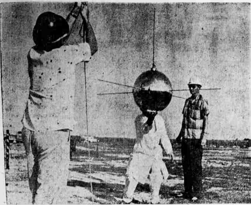
CHECK-OUT —Engineers hoist a 20" satellite aloft for a last check before placing it in the nose of the Vanguard rocket to be launched at Cape Canaveral, Fla. Later the rocket's second stage failed to ignite and place the satellite in orbit.
