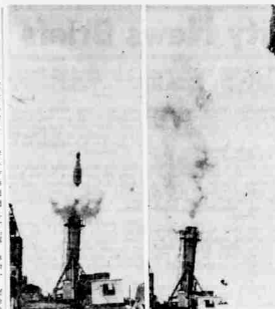
MISSILE LAUNCHER TESTED —Heavy cloud of smoke trails from mouth of prototype launcher (left) for the Navy's Polaris fleet ballistic missile during tests at San Francisco Naval Shipyard, Hunter's Point, Calif. At right, huge dummy missile made of concrete and steel can be seen falling toward San Francisco Bay after successful launch.
