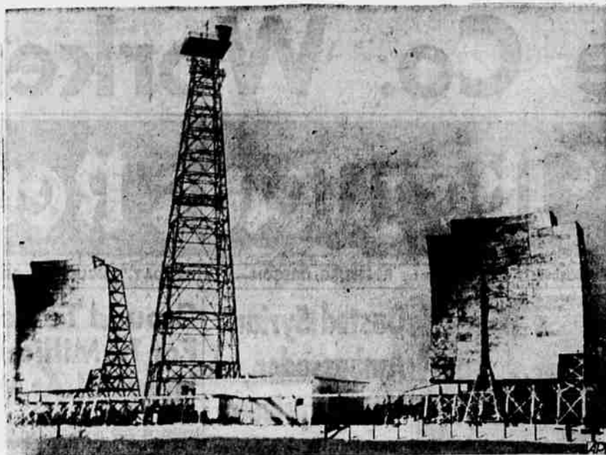
REFLECTORS BEAM INTERNATIONAL SIGNAL — Telephone signals over 185 miles of open water will soon be flashed from these giant 60-foot reflectors at Florida City, Fla., to similar equipment at Guanabo, Cuba. The signal, following a straight line and not the curvature of the earth, will strike a layer of air known as troposphere and be partially reflected downward to the receiving station. The new communications link will be established by the American Telephone and Telegraph Company and the Radio Corporation of Cuba. (AP)
