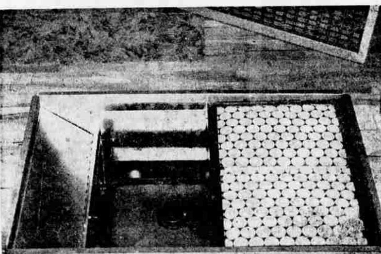
This is a "Cool Top" Floor Furnace With the Register Removed Showing Air Filter On Right
