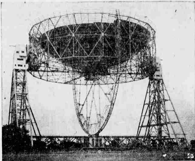
TO SEARCH THE STARS —The new radio telescope at Jodrell Bank, Eng. is ready for use during the International Geophysical Year. The 2,000-ton instrument, straddled on two supports which run on circular tracks, can detect stellar signals from any angle in space.
