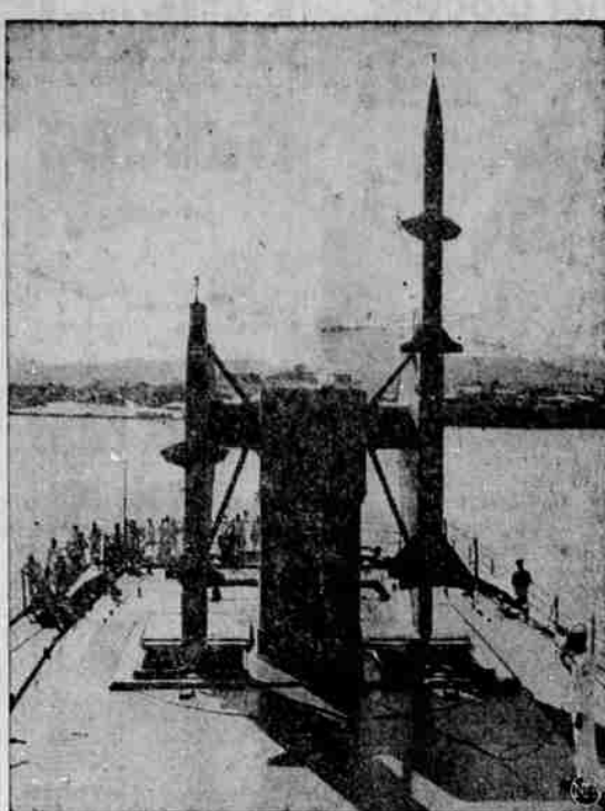
"READY ON THE RIGHT" — A "Terrier" guided missile, right, rises from the hold of the USS Boston and is received by a completely automatic guided-missile loading device. Stowage of the "Terrier" is below decks in two magazines, which operate similarly to automatic beverage-vending machines. At right is Seaman Leroy Steele of Akron, Ohio, directing the missile-placing by microphone. Another missile, left, is halfway out of the hold. USS Boston, the Navy's first guided-missile ship, will be sent to the critical Mediterranean area.
