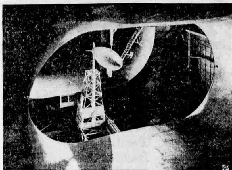
WIND INSTEAD OF WATER A one-fifth scale model of the submarine Albacore hangs in a wind tunnel at the National Advisory Committee for Aeronautics at Langley Field, Va. NACA scientists conducted this unusual experiment to help the Navy improve hull contour. The Navy announced its future atomic and conventional-powered subs will have the same shape as the Albacore, reputed to be the world's fastest submarine. (AP Wirephoto)
