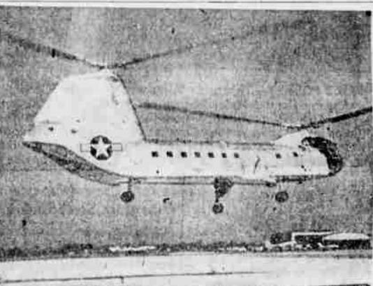
WORLD'S LARGEST 'COPTER —The world's largest jet powered transport helicopter, the 40-passenger Piasecki YH16A, made its debut this week. Known as the Turbo Transporter, it weighs more than 16 tons and has a top speed of about 150 miles an hour. Its 80-foot length makes it big enough to carry three jeeps. (AP WIREPHOTO)
