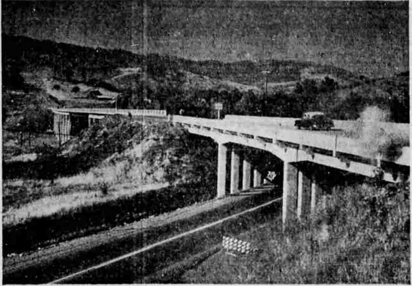
RIVER, HIGHWAY AND RAILROAD are crossed by new highway at Shady, the southern end of the bypass. The 946-foot bridge in background was the last link in construction of the $4,250,000 project.
