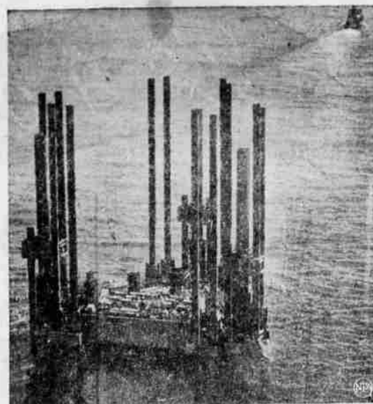
FIRST OF ITS KIND —Nearing its permanent location off the New England coast is the first of a series of offshore radar stations which will form a part of the U.S. continental defense system. The 6000-ton Texas-tower-type structure was anchored on George's Bank, some 100 miles out in the Atlantic. The man-made "island" is being pulled by a tug.
