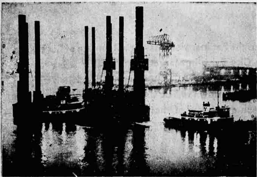
NATION'S FIRST —The nation's first floating radar island, a six thousand ton "Texas Tower," is shown as it was moved from its berth at the Fore River Shipyard in Quincy, Mass. The weird-looking island is being towed to Boston for further outfitting. Eventually it will be towed one hundred miles east of Cape Cod where it will stand on still-like legs 87 feet above water as part of the Continental Radar Warning System.
