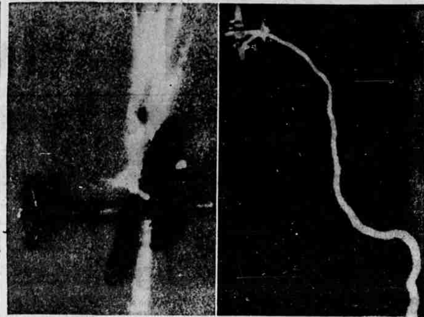
CAN'T MISS—The U. S. Air Force's "Falcon," a guided aircraft rocket, scores a direct hit on a QB-17 jet plane (left) after being fired from ground during tests. At right is view showing trail of smoke the Falcon left on its path to the target. The Falcon is the smallest guided missile in production and will be carried in quantity by USAF interceptor planes. In spite of its size, the rocket carries its own guidance system and its warhead can destroy a bomber. U. S. Air Force photo from NEA Telephoto.
