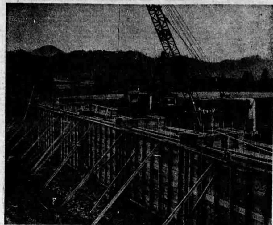
LOG POND BULKHEAD is being completed at Dixonville, where Roseburg Lumber Co. is constructing a green end to feed new plywood expansion at company's Dillard plant. Peeler, chain and other facilities will be housed in building to be constructed on far side of dike. Log pond is on camera side of bulkhead. (Paul Jenkins photo)
