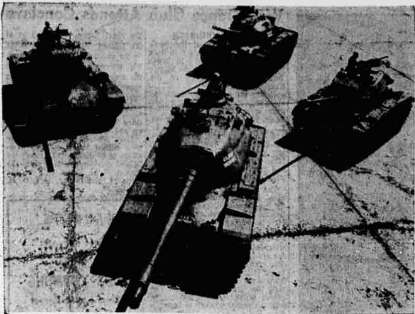
POWERED PACKED ARMY STEEDS —This is the first released view of the whole "family" of modern post World War II tanks designed by Army Ordnance for the ground forces. In foreground is heavy tank T-43 mounting a 120 mm. high velocity gun, largest ever mounted on a U. S. tank. Background, left to right: Medium gun tank M-47, medium gun tank M-48 and light gun tank M-41.
