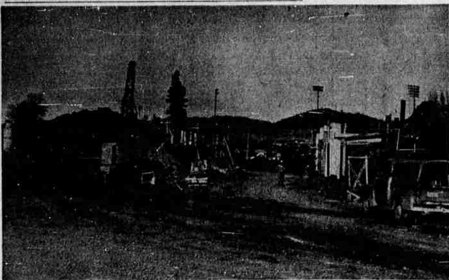
ANOTHER OVERPASS on the Pacific Highway rerouting through Roseburg is the Community Hospital Overpass above. Columns are being constructed now on Bellows Ave. by the R. E. Meade Co. of Grants Pass. The overpass will be 120 feet long and carry four lanes of traffic on its 58-foot width. It is comparable to the Harvard Street overpass, also located in West Roseburg. (Paul Jenkins Picture).
