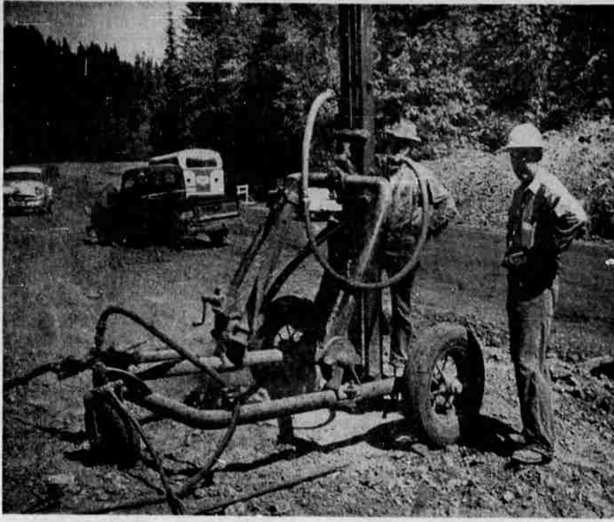
PREPARE TO BLAST — An automatic drill bores into a table of hardrock which will be blasted off to make way for the new section of Highway 99 about nine miles north of Drain. Traffic is already using the new roadbed on this section of the huge Divide-Rice Hill project. This work is part of the master plan to turn Pacific Highway from Eugene to the California border into a sleek, high-speed traffic tann. (Picture by Paul Jenkins)
