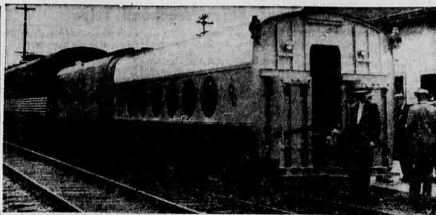
NEW RAILROAD CAR EXHIBITED —Representatives of 15 major United States and Canadian railroads were on hand to inspect this new type railroad passenger car shown in Detroit by the Chesapeake and Ohio railroad. One-third the usual coach length, the 31-foot low slung car has wheels on only one end. The wheel-less end attaches to the coach ahead. The car floor is 2½ feet closer to the ground than the usual coach. The roof is three feet lower. (AP Wirephoto)
